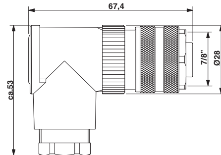
7/8" female connector, angled
