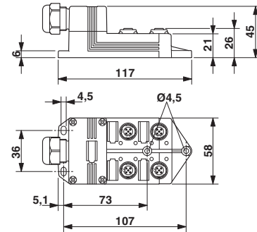
Dimensioned drawing
