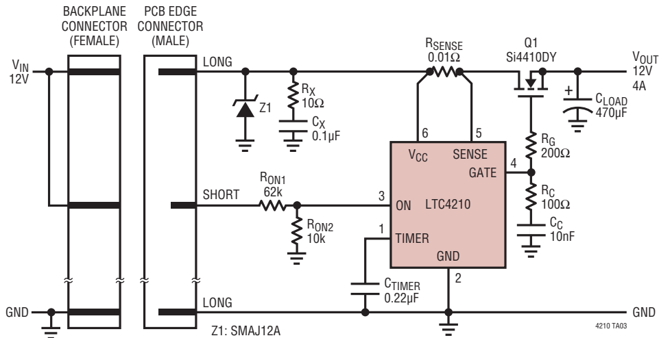
12V Hot Swap Application
