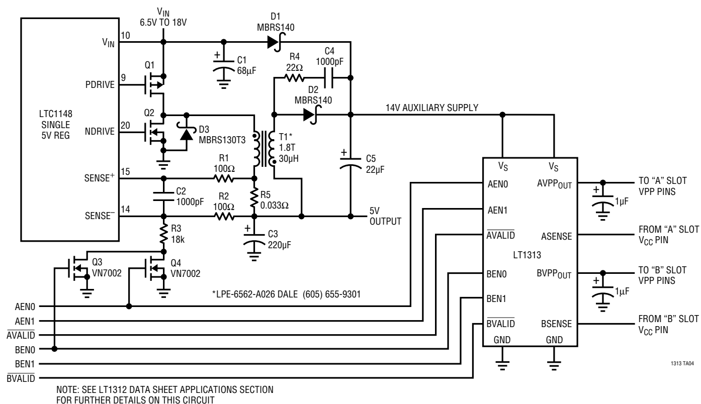
Dual Slot PCMCIA Driver/Regulator Powered from Auxiliary Winding on 5V Inductor of LTC1142HV Dual 5V/3.3V Switching Regulator
