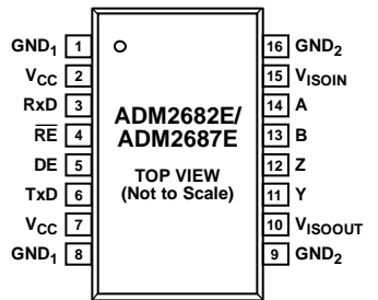
Figure 2. Pin Configuration
