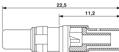
Dimensioned drawing
