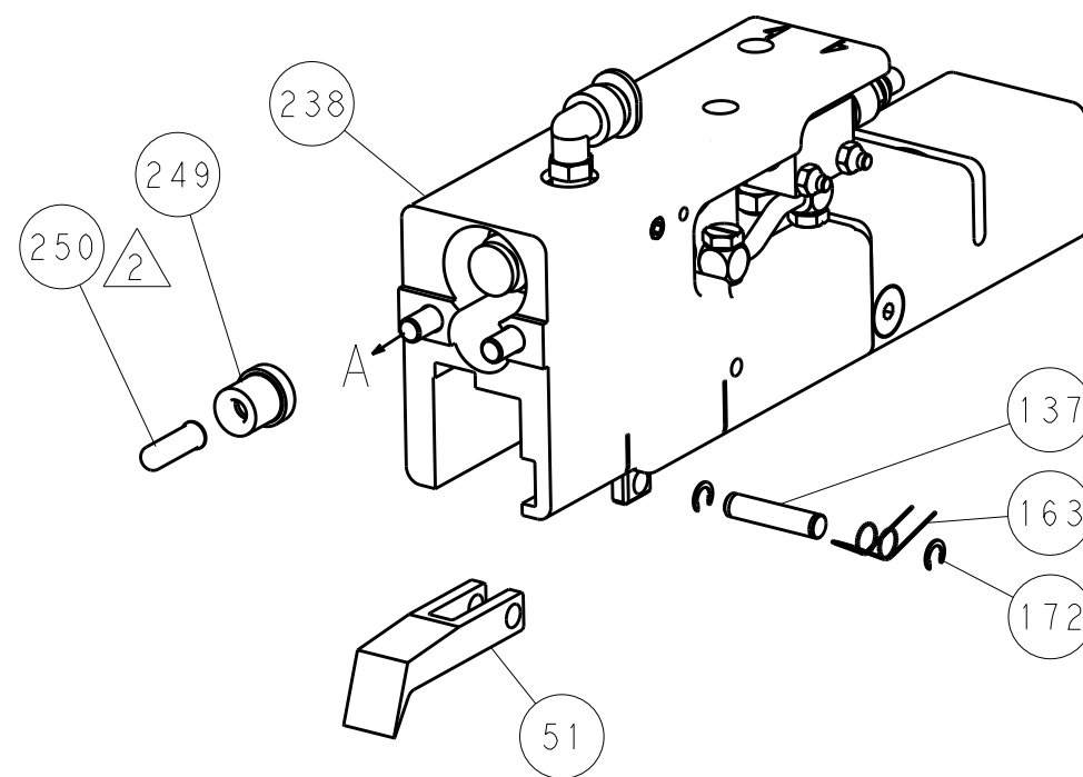
PNEUMATIC
