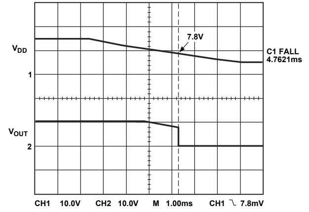
Figure 13. Turn-Off Characteristics
