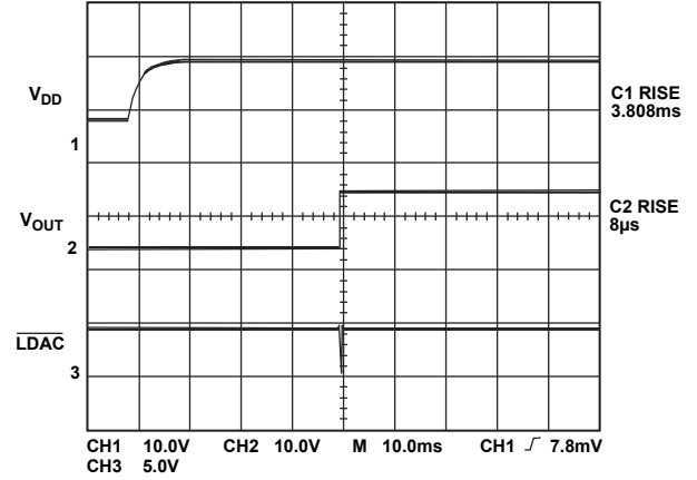
Figure 12. Turn-On Characteristics
