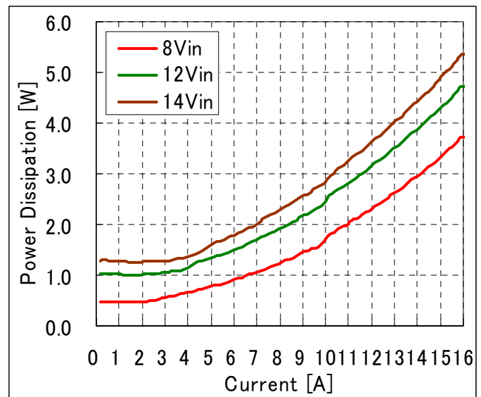
Fig-5.0V-3: Power Loss vs. load current and input voltage for V_{out}=5.0V . Airflow rate=200 LFM (1m/s) and T_a=25^{\circ}C .
