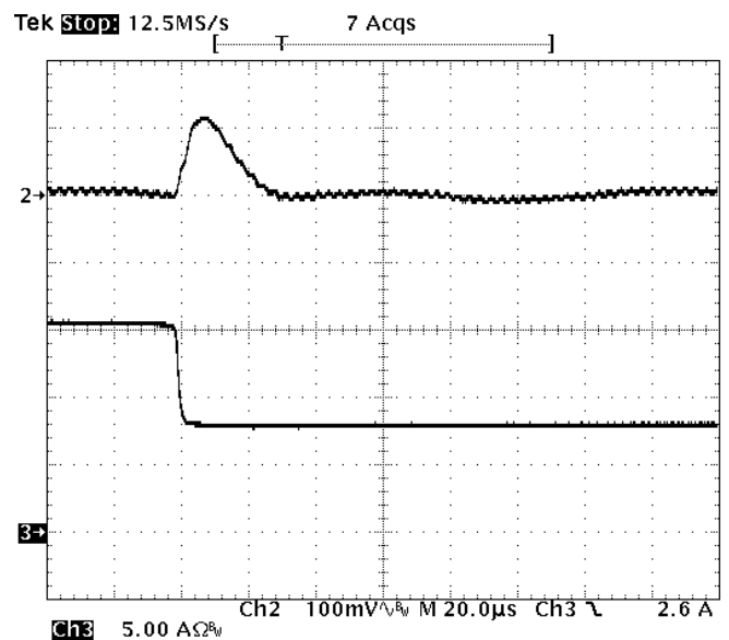
Fig-1.2V-7: Output voltage response for V_{out}=1.2V to negative load current step change from 16A to 8A with slew rate of -5A/us at V_{in}=12V . C_o=47\mu F \times 4 ceramic. Top trace: output voltage (100mV/div.) Bottom trace: load current (5A/div.) Time scale: 20us/div.
