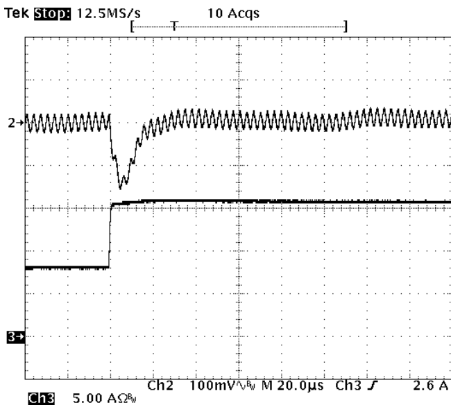
Fig-5.0V-6: Output voltage response for V_{out}=5.0V to positive load current step change from 8A to 16A with slew rate of 5A/us at V_{in}=12V . C_o=47\mu F \times 4 ceramic. Top trace: output voltage (100mV/div.) Bottom trace: load current (5A/div.) Time scale: 20us/div.
