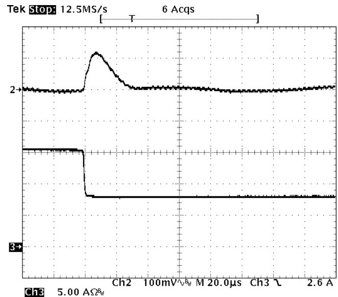
Fig-1.0V-7: Output voltage response for V_{out}=1.0V to negative load current step change from 16A to 8A with slew rate of -5A/\mu s at V_{in}=12V . C_o=47\mu F \times 4 ceramic. Top trace: output voltage (100mV/div.) Bottom trace: load current (5A/div.) Time scale: 20us/div.
