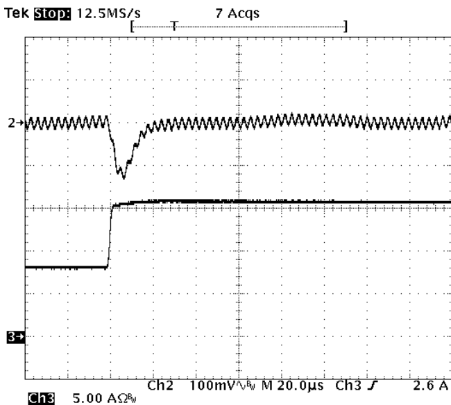
Fig-3.3V-6: Output voltage response for V_{out}=3.3V to positive load current step-change from 8A to 16A with slew rate of 5A/us at V_{in}=12V . C_o=47uFx4 ceramic. Top trace: output voltage (100mV/div.) Bottom trace: load current (5A/div.) Time scale: 20us/div.
