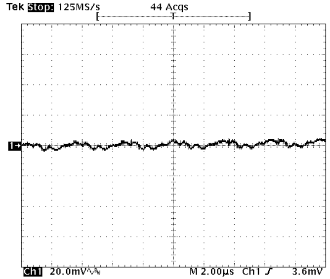
Fig-1.8V-5: Output voltage ripple (20mV/div.) for V_{out}=1.8V at full rated load current into a resistive load with external capacitance 47\mu F \times 4 ceramic + 1\mu F ceramic at V_{in}=12V . Time scale: 2 us/div
