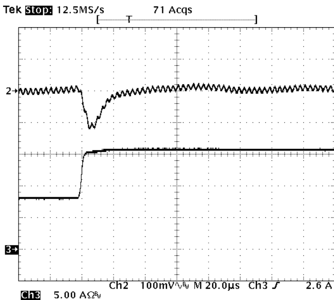
Fig-2.5V-6: Output voltage response for V_{out}=2.5V to positive load current step change from 8A to 16A with slew rate of 5A/us at V_{in}=12V . C_o=47uF \times 4 ceramic. Top trace: output voltage (100mV/div.) Bottom trace: load current (5A/div.) Time scale: 20us/div.
