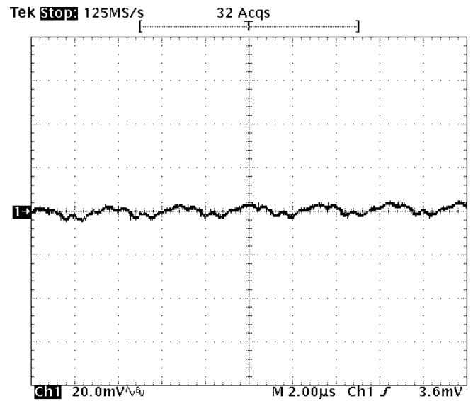
Fig-2.0V-5: Output voltage ripple (20mV/div.) for V_{out}=2.0V at full rated load current into a resistive load with external capacitance 47\mu F \times 4 ceramic + 1\mu F ceramic at V_{in}=12V . Time scale: 2 us/div
