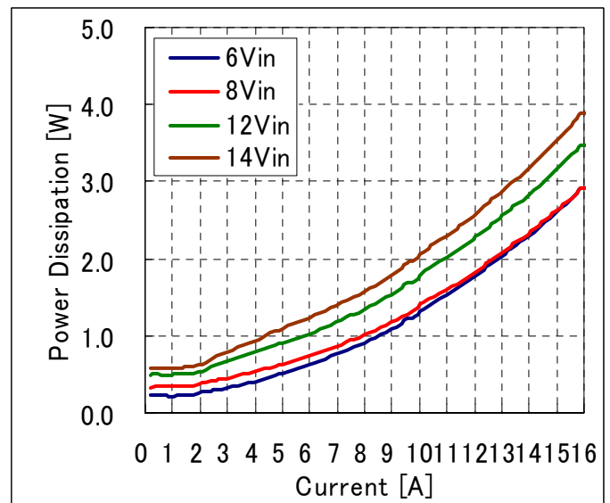
Fig-1.8V-3: Power Loss vs. load current and input voltage for V_{out}=1.8V . Airflow rate=200 LFM (1m/s) and T_a=25^{\circ}C .
