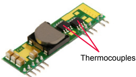
Fig. D: Location of the thermocouples for thermal testing
