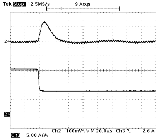
Fig-1.5V-7: Output voltage response for V_{out}=1.5V to negative load current step change from 16A to 8A with slew rate of -5A/\mu s at V_{in}=12V . C_o=47\mu F \times 4 ceramic. Top trace: output voltage (100mV/div.) Bottom trace: load current (5A/div.) Time scale: 20us/div.
