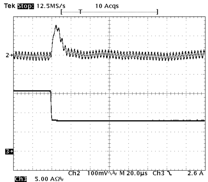
Fig-5.0V-7: Output voltage response for V_{out}=5.0V to negative load current step change from 16A to 8A with slew rate of -5A/us at V_{in}=12V . C_o=47\mu F \times 4 ceramic. Top trace: output voltage (100mV/div.) Bottom trace: load current (5A/div.) Time scale: 20us/div.
