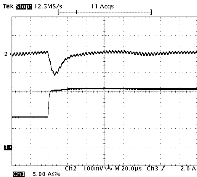
Fig-2.0V-6: Output voltage response for V_{out}=2.0V to positive load current step change from 8A to 16A with slew rate of 5A/\mu s at V_{in}=12V . C_o=47\mu F \times 4 ceramic. Top trace: output voltage (100mV/div.) Bottom trace: load current (5A/div.) Time scale: 20us/div.
