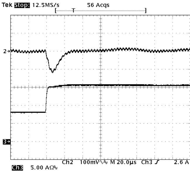
Fig-1.8V-6: Output voltage response for V_{out}=1.8V to positive load current step change from 8A to 16A with slew rate of 5A/\mu s at V_{in}=12V . C_o=47\mu F \times 4 ceramic. Top trace: output voltage (100mV/div.) Bottom trace: load current (5A/div.) Time scale: 20us/div.
