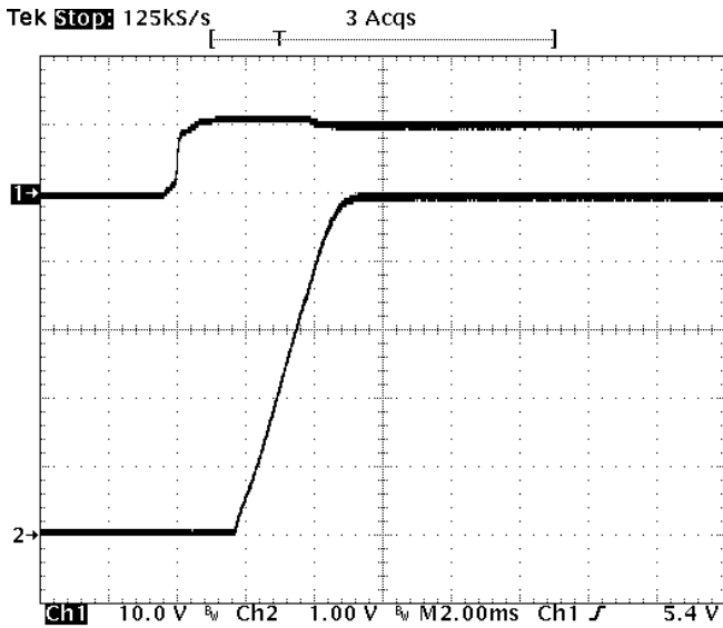
Fig-5.0V-4: Turn-on transient for V_{out}=5.0V with application of V_{in} at full rated load current (resistive) and 47\mu F \times 4 external capacitance at V_{in}=12V . Top trace: V_{in} (10V/div.) Bottom trace: output voltage (1V/div.) Time scale: 2 ms/div.
