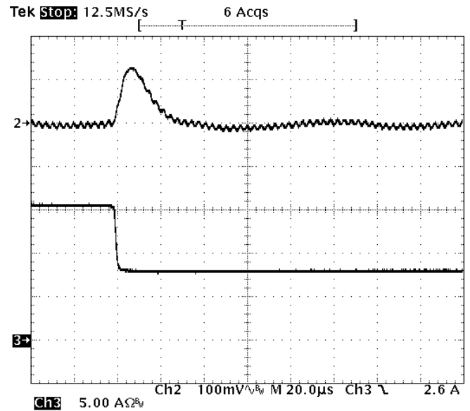
Fig-1.8V-7: Output voltage response for V_{out}=1.8V to negative load current step change from 16A to 8A with slew rate of -5A/\mu s at V_{in}=12V . C_o=47\mu F \times 4 ceramic. Top trace: output voltage (100mV/div.) Bottom trace: load current (5A/div.) Time scale: 20us/div.
