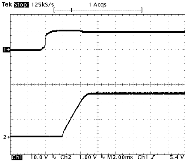
Fig-2.5V-4: Turn-on transient for V_{out}=2.5V with application of V_{in} at full rated load current (resistive) and 47uF \times 4 external capacitance at V_{in}=12V . Top trace: V_{in} (10V/div.) Bottom trace: output voltage (1V/div.) Time scale: 2 ms/div.
