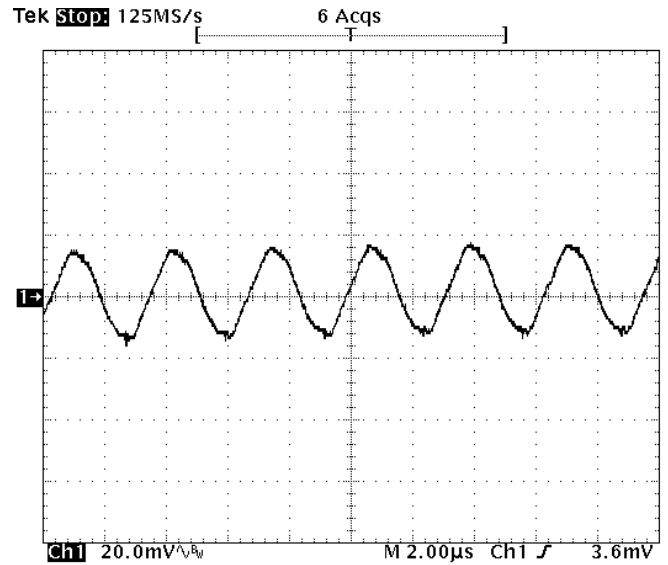
Fig-5.0V-5: Output voltage ripple (20mV/div.) for V_{out}=5.0V at full rated load current into a resistive load with external capacitance 47\mu F \times 4 ceramic + 1uF ceramic at V_{in}=12V . Time scale: 2 us/div
