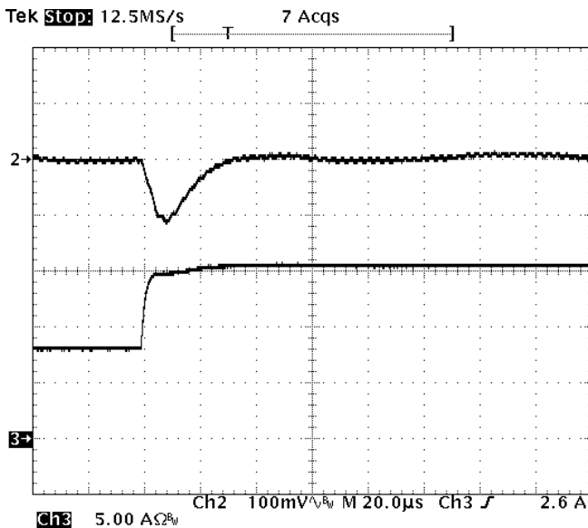
Fig-1.0V-6: Output voltage response for V_{out}=1.0V to positive load current step change from 8A to 16A with slew rate of 5A/\mu s at V_{in}=12V . C_o=47\mu F \times 4 ceramic. Top trace: output voltage (100mV/div.) Bottom trace: load current (5A/div.) Time scale: 20us/div.
