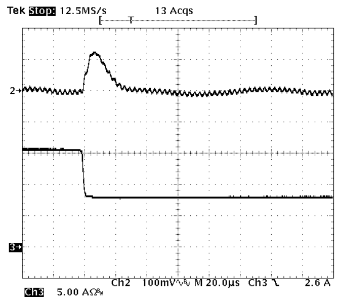
Fig-2.0V-7: Output voltage response for V_{out}=2.0V to negative load current step change from 16A to 8A with slew rate of -5A/\mu s at V_{in}=12V . C_o=47\mu F \times 4 ceramic. Top trace: output voltage (100mV/div.) Bottom trace: load current (5A/div.) Time scale: 20us/div.
