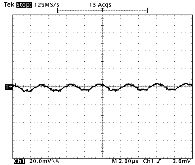
Fig-2.5V-5: Output voltage ripple (20mV/div.) for V_{out}=2.5V at full rated load current into a resistive load with external capacitance 47uF \times 4 ceramic + 1uF ceramic at V_{in}=12V . Time scale: 2 us/div
