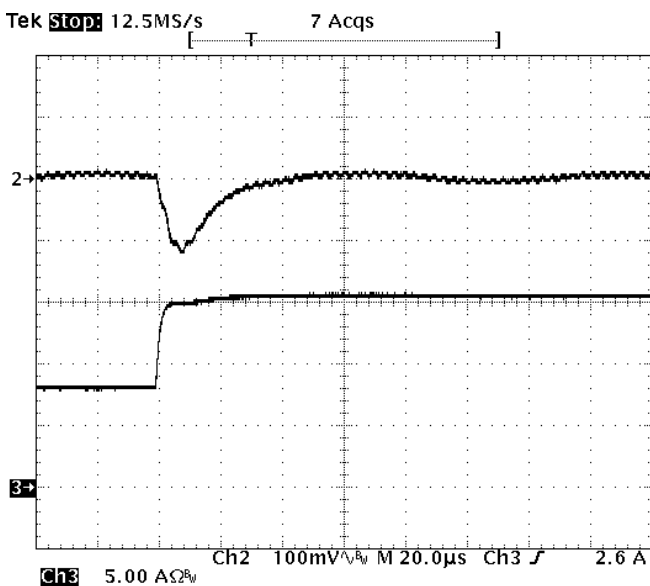
Fig-1.2V-6: Output voltage response for V_{out}=1.2V to positive load current step change from 8A to 16A with slew rate of 5A/us at V_{in}=12V . C_o=47\mu F \times 4 ceramic. Top trace: output voltage (100mV/div.) Bottom trace: load current (5A/div.) Time scale: 20us/div.
