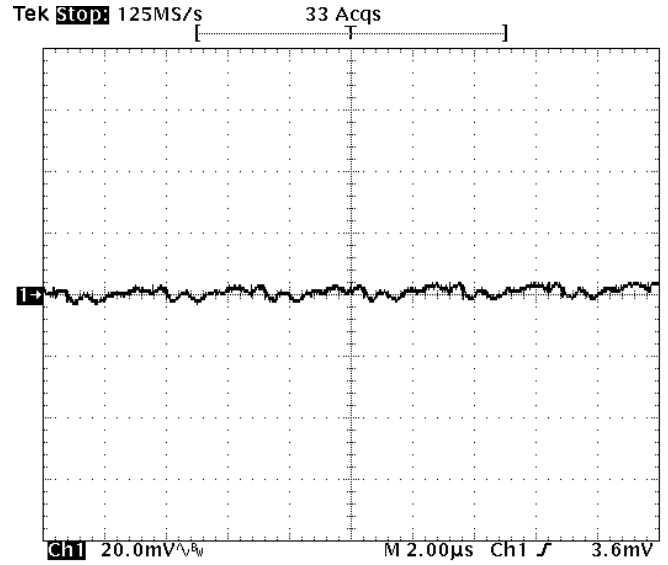
Fig-1.5V-5: Output voltage ripple (20mV/div.) for V_{out}=1.5V at full rated load current into a resistive load with external capacitance 47\mu F \times 4 ceramic + 1\mu F ceramic at V_{in}=12V . Time scale: 2us/div
