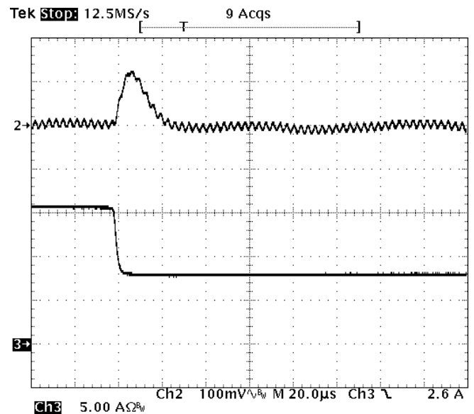
Fig-2.5V-7: Output voltage response for V_{out}=2.5V to negative load current step change from 16A to 8A with slew rate of -5A/us at V_{in}=12V . C_o=47uF \times 4 ceramic. Top trace: output voltage (100mV/div.) Bottom trace: load current (5A/div.) Time scale: 20us/div.
