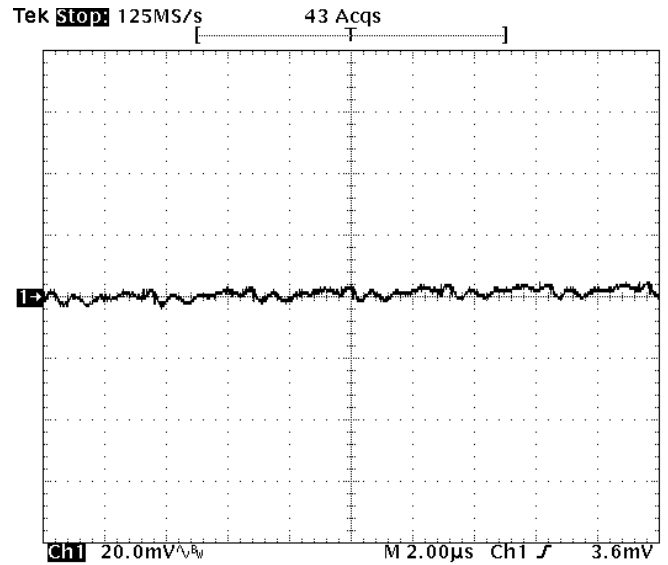
Fig-1.2V-5: Output voltage ripple (20mV/div.) for V_{out}=1.2V at full rated load current into a resistive load with external capacitance 47\mu F \times 4 ceramic + 1\mu F ceramic at V_{in}=12V . Time scale: 2us/div
