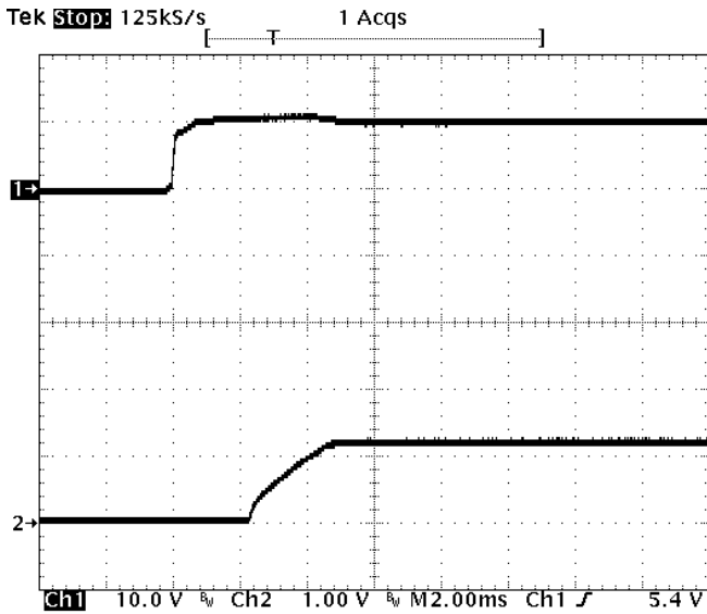
Fig-1.2V-4: Turn-on transient for V_{out}=1.2V with application of V_{in} at full rated load current (resistive) and 47\mu F \times 4 external capacitance at V_{in}=12V . Top trace: V_{in} (10V/div.) Bottom trace: output voltage (1V/div.) Time scale: 2ms/div.
