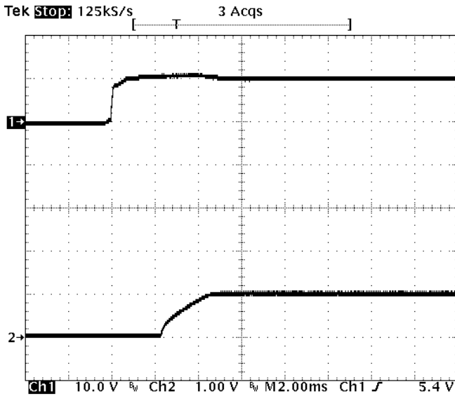
Fig-1.0V-4: Turn-on transient for V_{out}=1.0V with application of V_{in} at full rated load current (resistive) and 47\mu F \times 4 external capacitance at V_{in}=12V . Top trace: V_{in} (10V/div.) Bottom trace: output voltage (1V/div.) Time scale: 2 ms/div.
