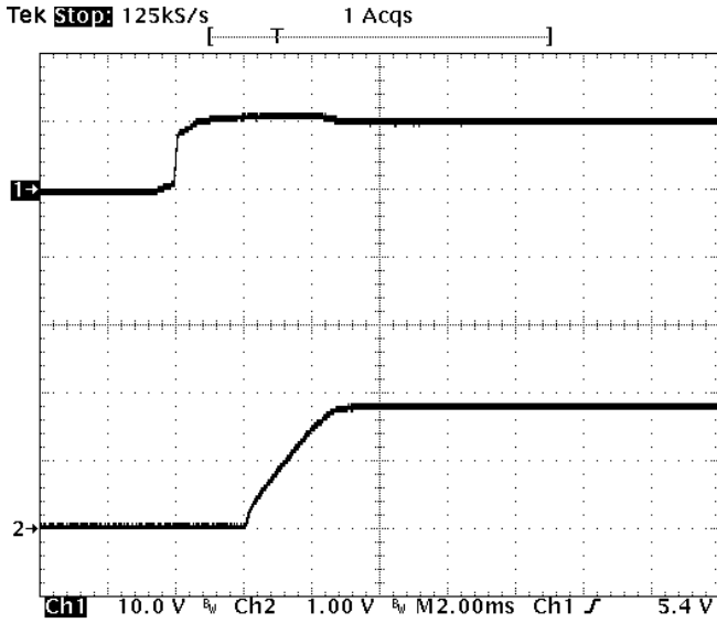
Fig-1.8V-4: Turn-on transient for V_{out}=1.8V with application of V_{in} at full rated load current (resistive) and 47\mu F \times 4 external capacitance at V_{in}=12V . Top trace: V_{in} (10V/div.) Bottom trace: output voltage (1V/div.) Time scale: 2 ms/div.
