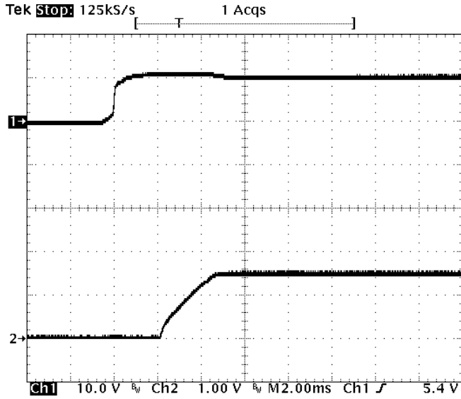
Fig-1.5V-4: Turn-on transient for V_{out}=1.5V with application of V_{in} at full rated load current (resistive) and 47\mu F \times 4 external capacitance at V_{in}=12V . Top trace: V_{in} (10V/div.) Bottom trace: output voltage (1V/div.) Time scale: 2 ms/div.
