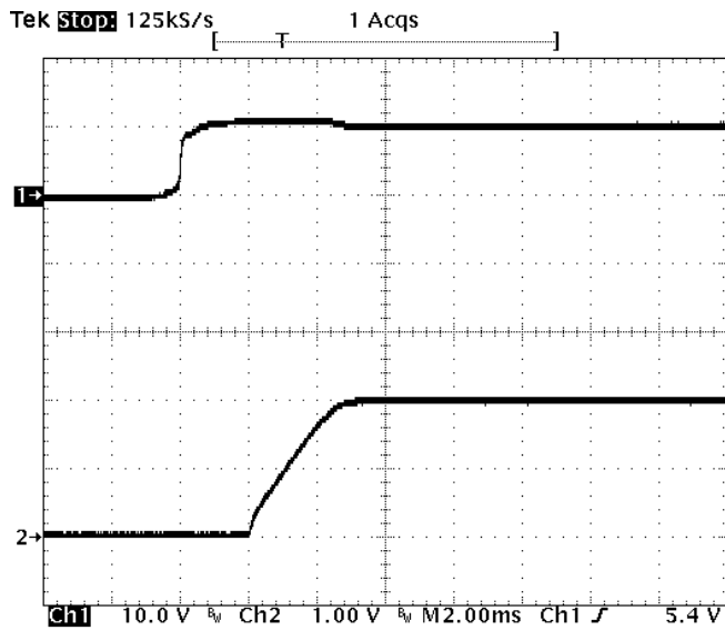
Fig-2.0V-4: Turn-on transient for V_{out}=2.0V with application of V_{in} at full rated load current (resistive) and 47\mu F \times 4 external capacitance at V_{in}=12V . Top trace: V_{in} (10V/div.) Bottom trace: output voltage (1V/div.) Time scale: 2 ms/div.
