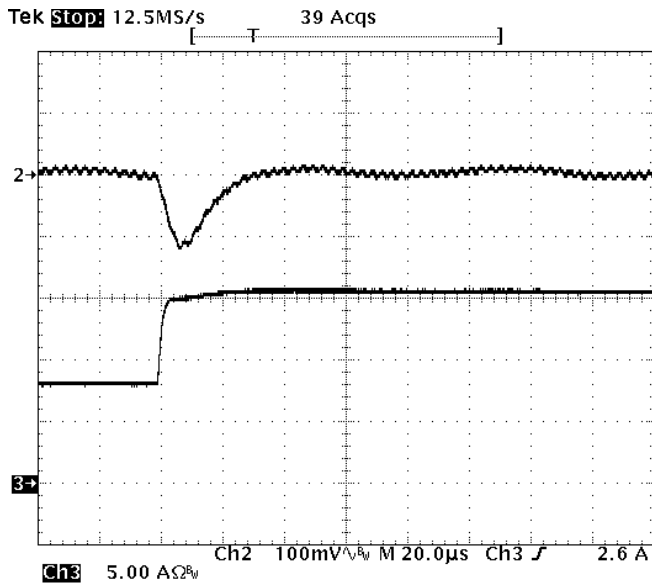
Fig-1.5V-6: Output voltage response for V_{out}=1.5V to positive load current step change from 8A to 16A with slew rate of 5A/\mu s at V_{in}=12V . C_o=47\mu F \times 4 ceramic. Top trace: output voltage (100mV/div.) Bottom trace: load current (5A/div.) Time scale: 20us/div.
