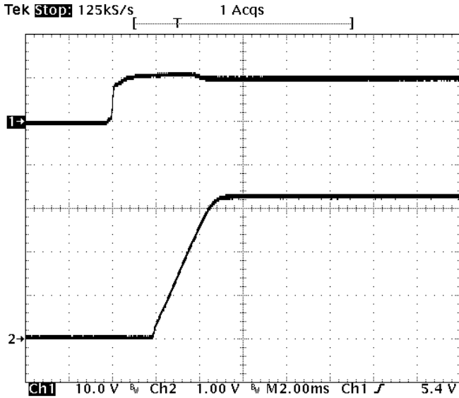
Fig-3.3V-4: Turn-on transient for V_{out}=3.3V with application of V_{in} at full rated load current (resistive) and 47uFx4 external capacitance at V_{in}=12V . Top trace: V_{in} (10V/div.) Bottom trace: output voltage (1V/div.) Time scale: 2ms/div.
