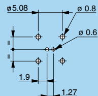
P19 - EPG-EXG (0B/1B.302) Screw mount
