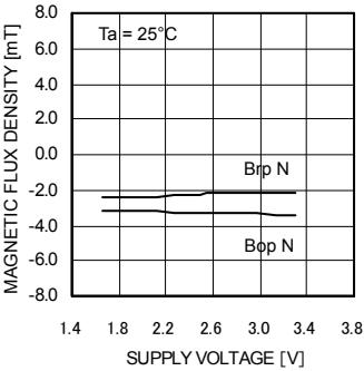
Fig.31 Bop,Brp – Supply voltage
