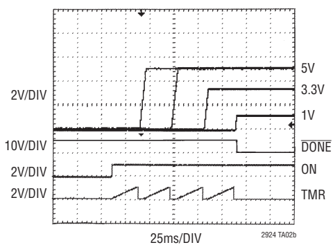
Power-Up Sequence
