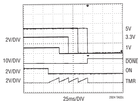
Power-Down Sequence
