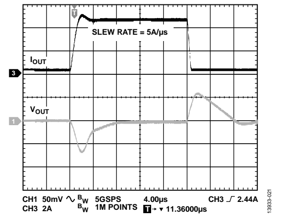
Figure 21. Load Transient Response, C_{OUT} = 47\mu F , V_{IN} = 1.8V , V_{OUT} = 1.3V
