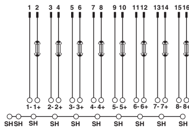
Connection scheme UM-DELTA V/D/SI
