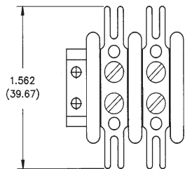
"W" Terminals
