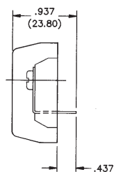
"Y" Terminals
