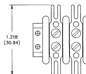
"W" Terminals
