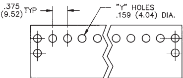
"Y" Terminal
