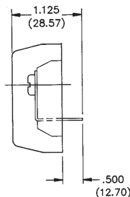
“Y” Terminals
