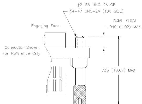
Standard Jackscrew
