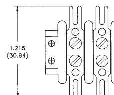
"W" Terminals
