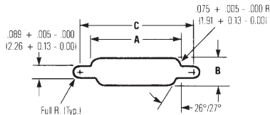
Rear Mounting
