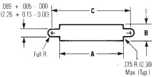
Front Mounting
