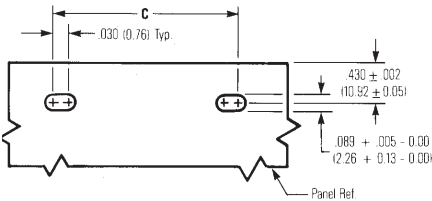
Edgeboard Mounting
