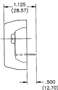
“Y” Terminals
