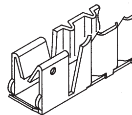
Termination section of IDC contact
