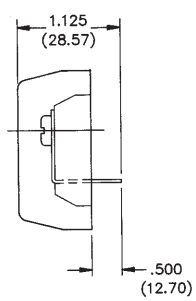
“Y” Terminals
