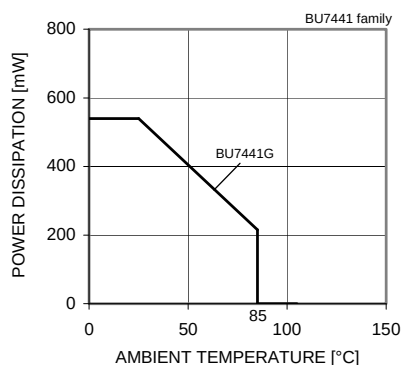
Fig.93 Derating curve
