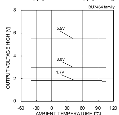
Fig.52 Output Voltage High - Ambient Temperature ( R_L=10[k\Omega] )
