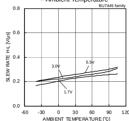
Fig.183 Slew Rate H-L – Ambient Temperature
