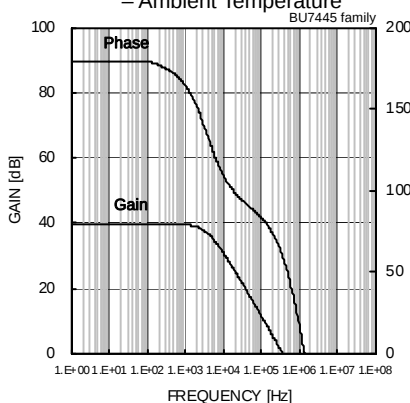
Fig.184 Gain – Frequency
