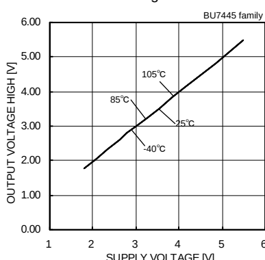
Fig.166 Output Voltage High – Supply Voltage (RL=10[kΩ])
