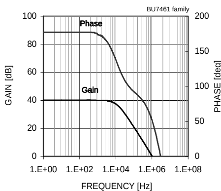
Fig.23 Gain – Frequency
