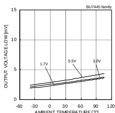
Fig.169 Output Voltage Low – Ambient Temperature (RL=10[kΩ])
