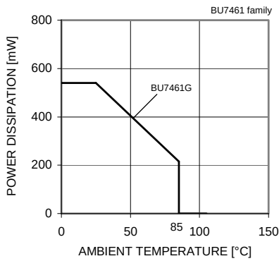
Fig.1 Derating curve
