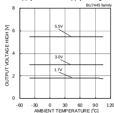
Fig.167 Output Voltage High – Ambient Temperature (RL=10[kΩ])
