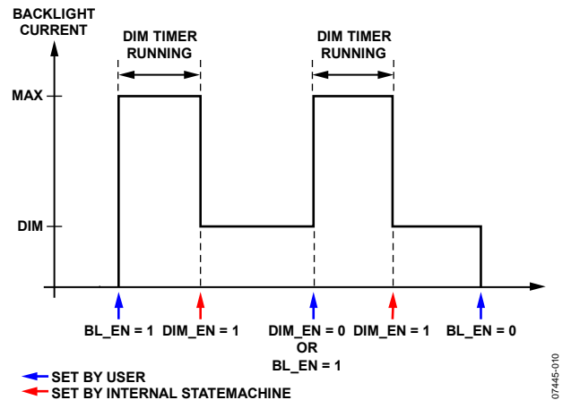
Figure 19. Dim Timer
