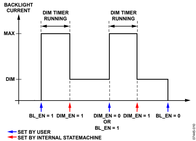
Figure 19. Dim Timer
