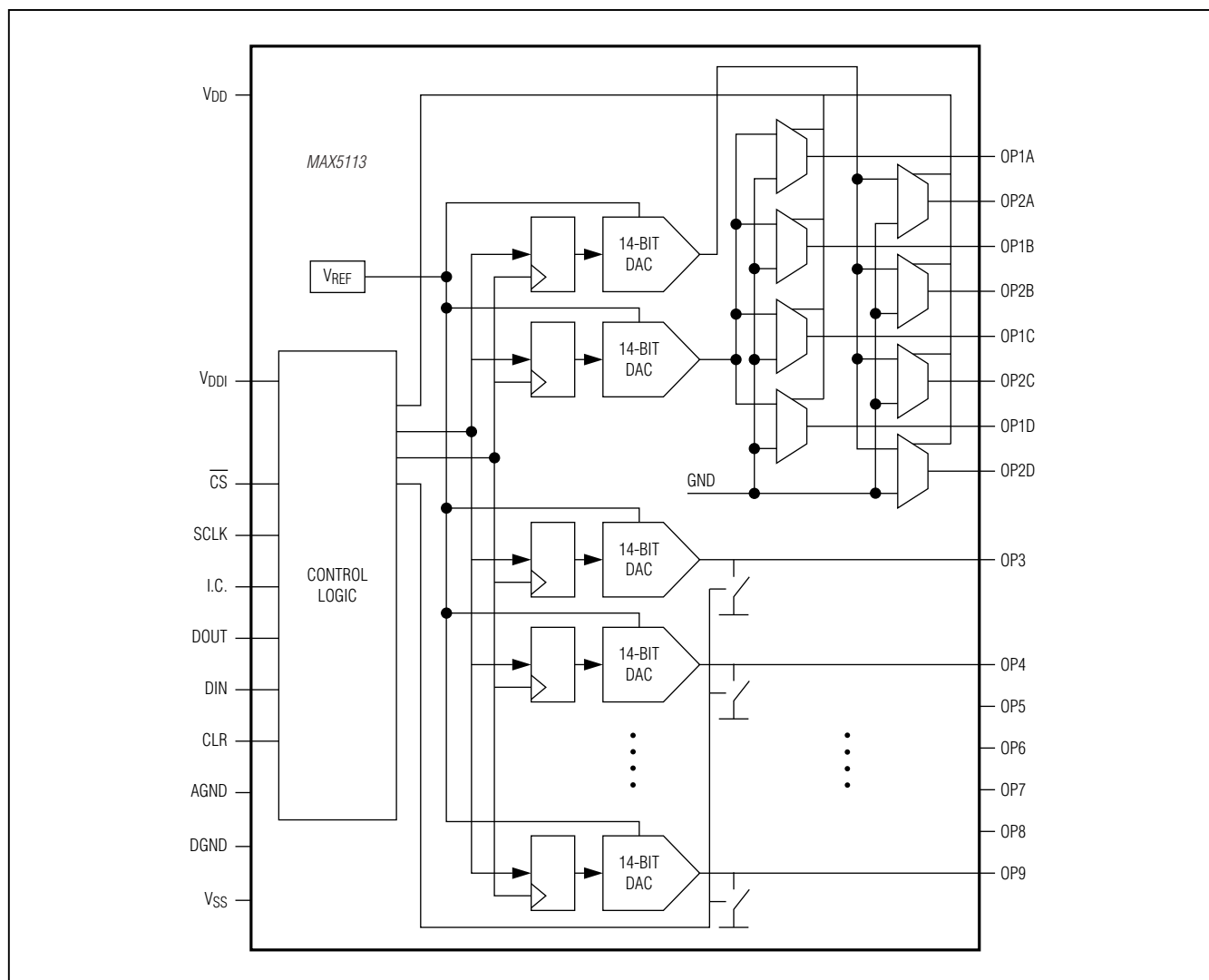
Functional Diagram
