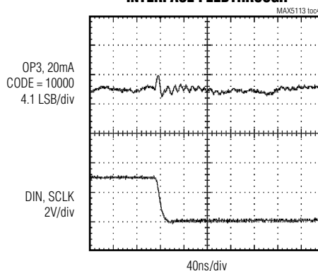
INTERFACE FEEDTHROUGH
