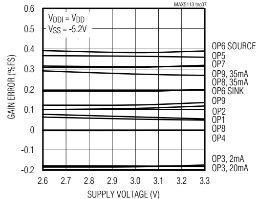
GAIN ERROR vs. ANALOG SUPPLY VOLTAGE
