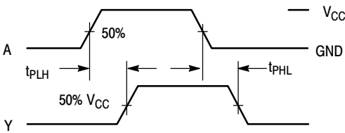
Figure 4. Switching Wave Forms
