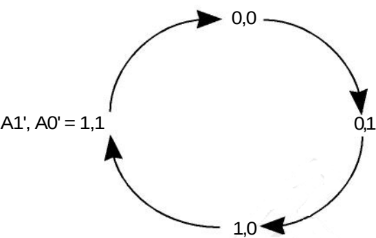
LINEAR BURST ADDRESS TABLE (MODE = V ss )
