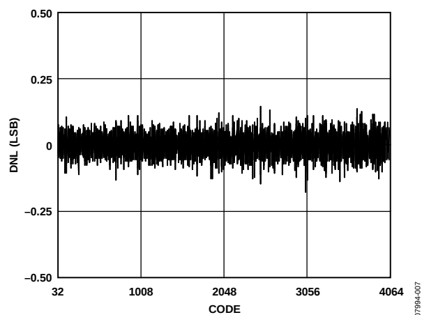
Figure 7. Typical DNL
