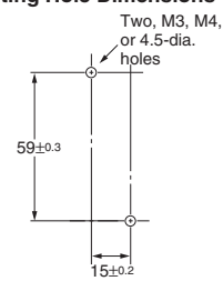
Mounting Hole Dimensions
