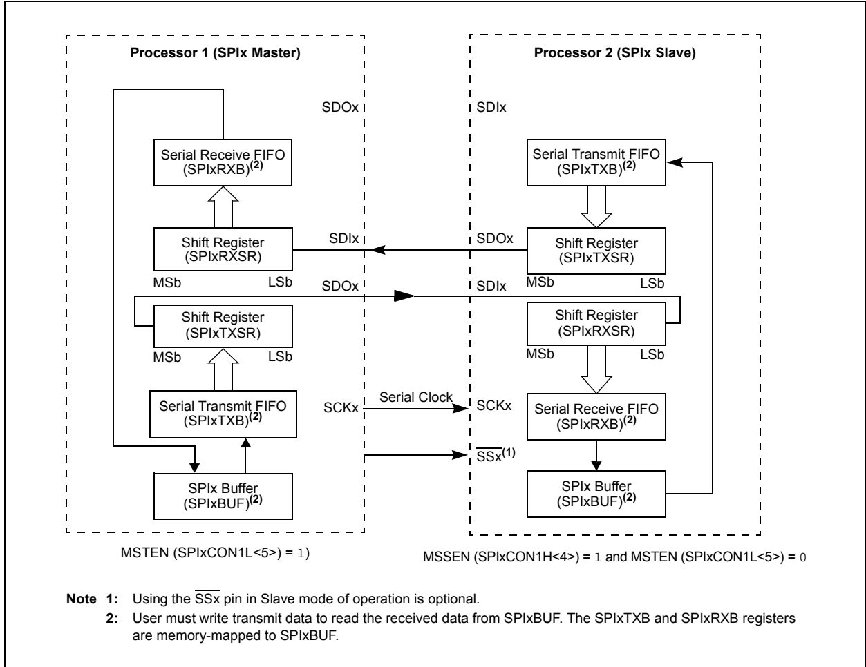
FIGURE 14-4: SPIx MASTER/S�AVE CONNECTION (ENHANCED BUFFER MODES)
