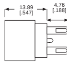
CONNECTOR 515-0074
