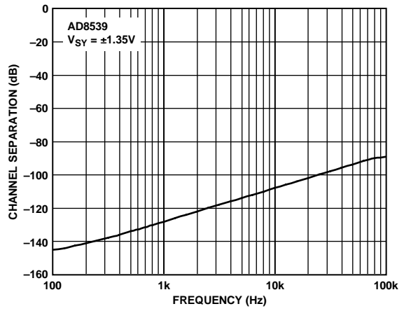
Figure 63. AD8539 Channel Separation vs. Frequency
