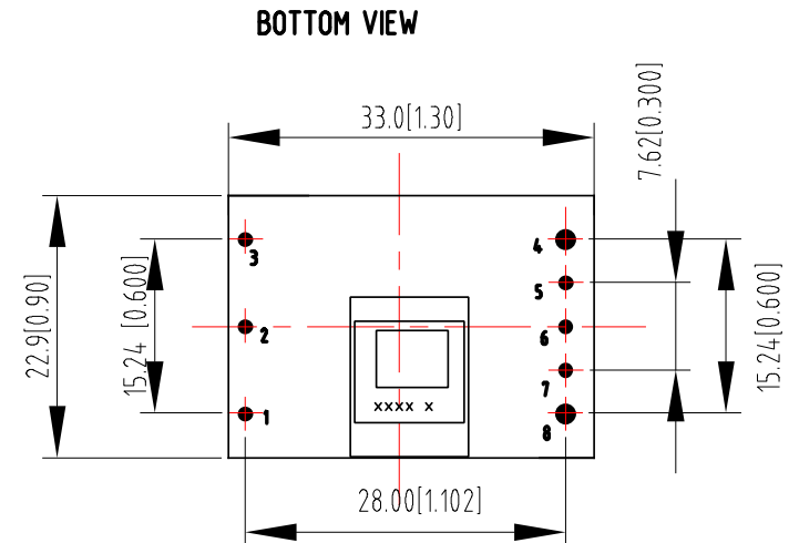
Model: AVD85B-48S05B-6L
