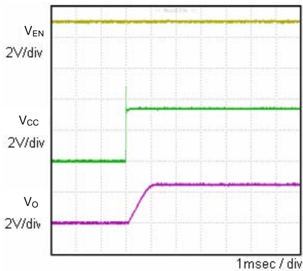
Fig.5 Input sequence1 Co=1.0μF
