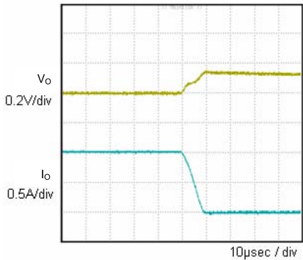
Fig.4 Transient Response(1.0→0A) Co=1.0μF
