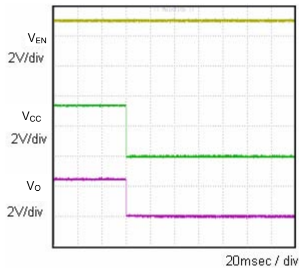
Fig.6 OFF sequence 1 Co=1.0μF
