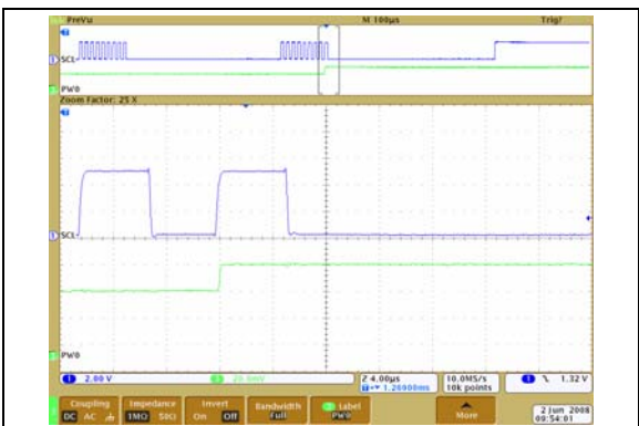
FIGURE 2-18: 5 k \Omega – Low-Voltage Increment Wiper Settling Time ( V_{DD} = 2.7V ) (1 \mu s /Div).
