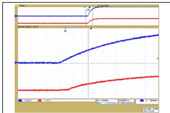
FIGURE 2-42: 50 k \Omega – Power-Up Wiper Response Time (1 \mu\text{s}/\text{Div} ).
