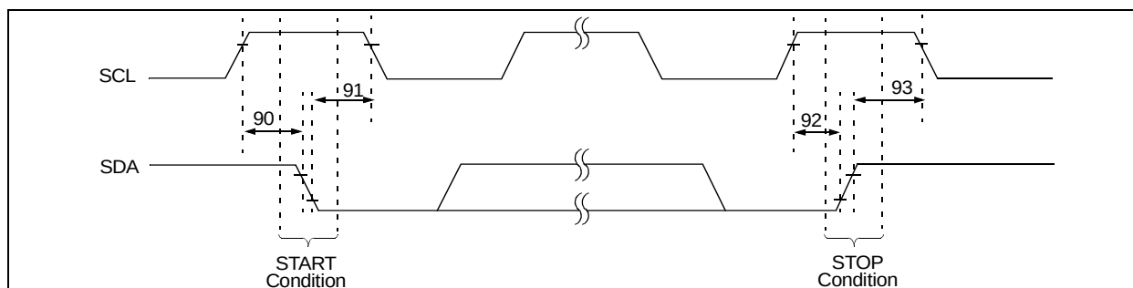
FIGURE 1-1: I^2\text{C} Bus Start/Stop Bits Timing Waveforms.
