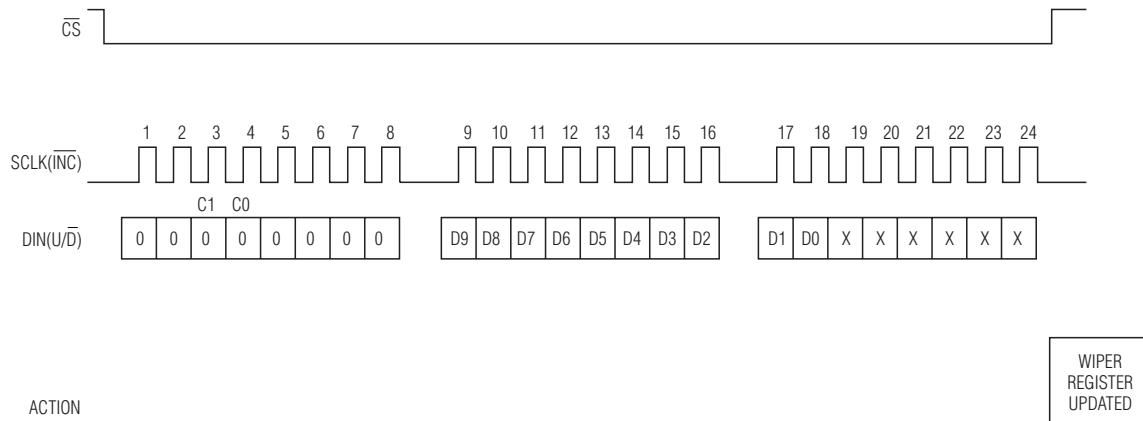
Figure 5. Write Wiper Register Operation
