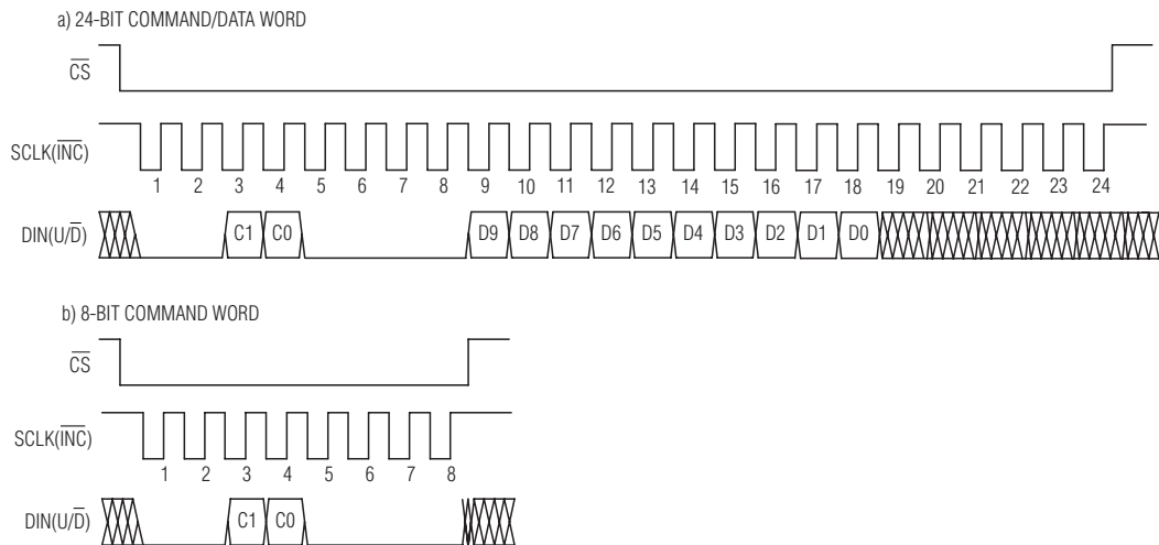
Figure 4. Serial SPI-Compatible Interface Format
