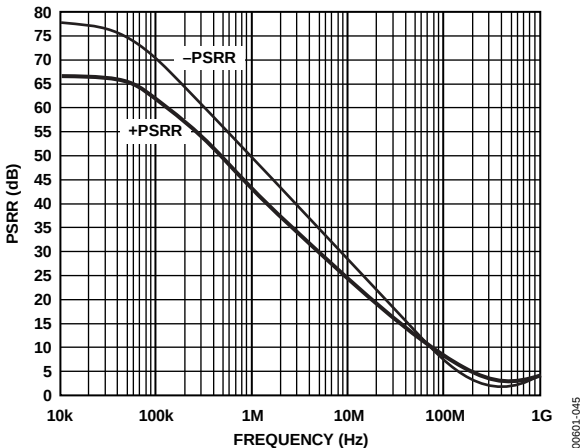
Figure 45. AD9632 PSRR vs. Frequency
