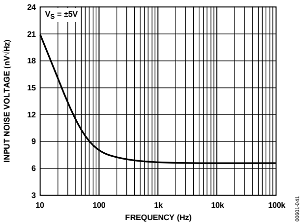
Figure 41. AD9631 Noise vs. Frequency
