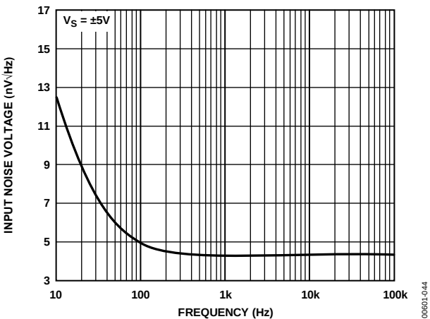
Figure 44. AD9632 Noise vs. Frequency
