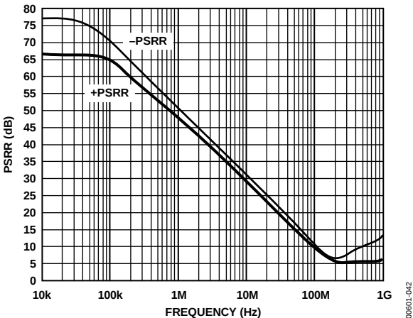
Figure 42. AD9631 PSRR vs. Frequency
