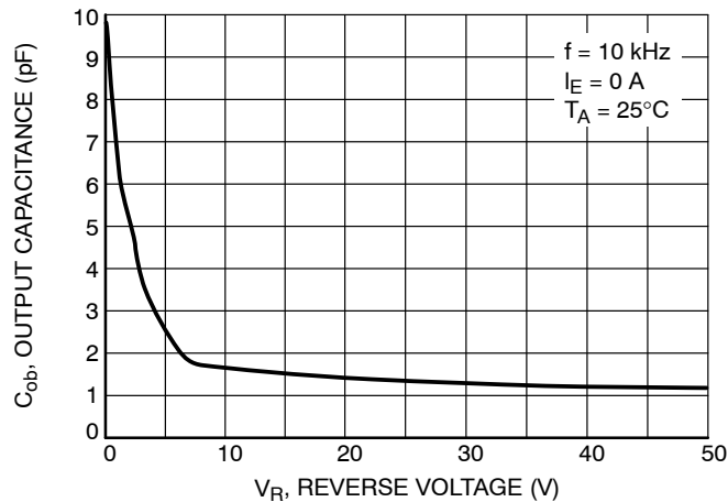
Figure 4. Output Capacitance
