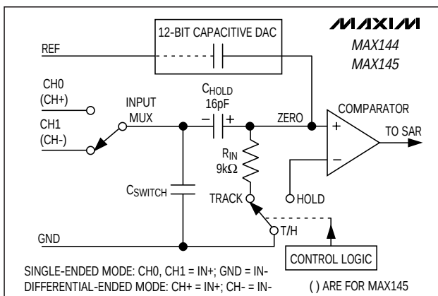
Figure 3. Analog Input Channel Structure
