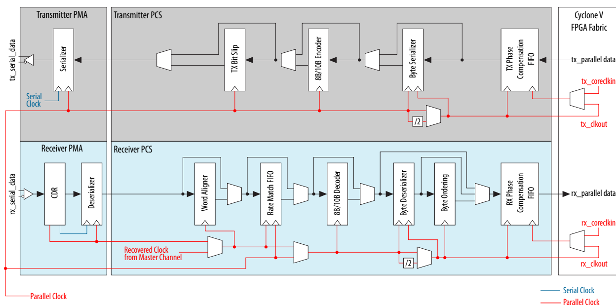
Figure 16-2: The Standard PCS Datapath
