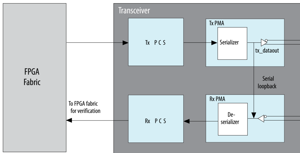
Figure 17-16: Serial Loopback
