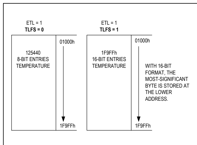
Figure 7. Temperature Logging
