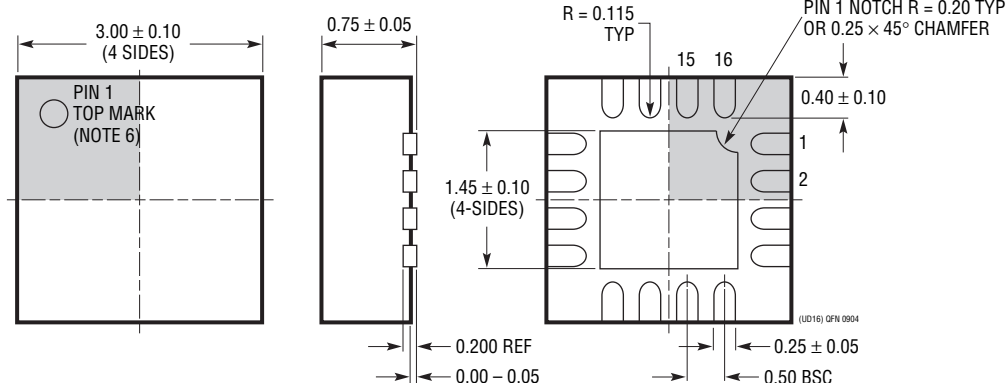
BOTTOM VIEW—EXPOSED PAD
