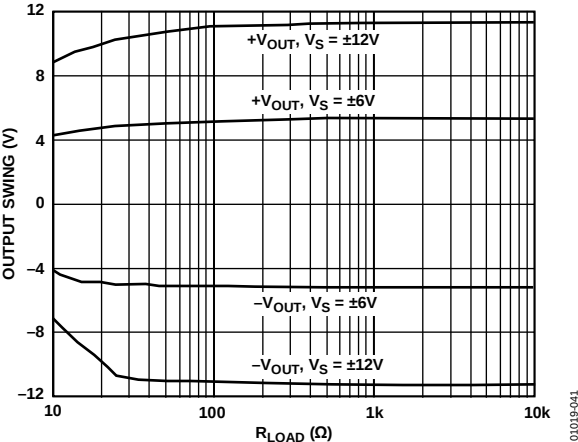
Figure 39. Output Voltage vs. R_{LOAD}
