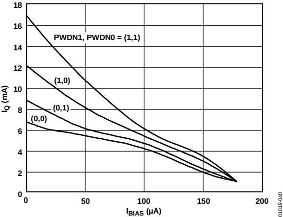
Figure 38. I_Q vs. I_{BIAS} Current; V_S = \pm 6V
