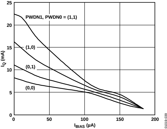
Figure 37. I_Q vs. I_{BIAS} Current; V_S = \pm 12V
