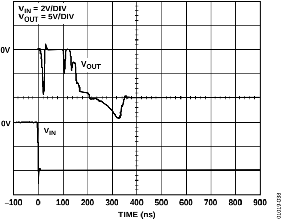
Figure 36. Negative Overdrive Recovery; V_S = \pm 12V , G = +5 , R_L = 100\Omega
