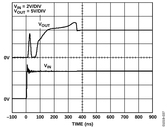
Figure 35. Positive Overdrive Recovery; V_S = \pm 12\text{ V} , G = +5 , R_L = 100\Omega
