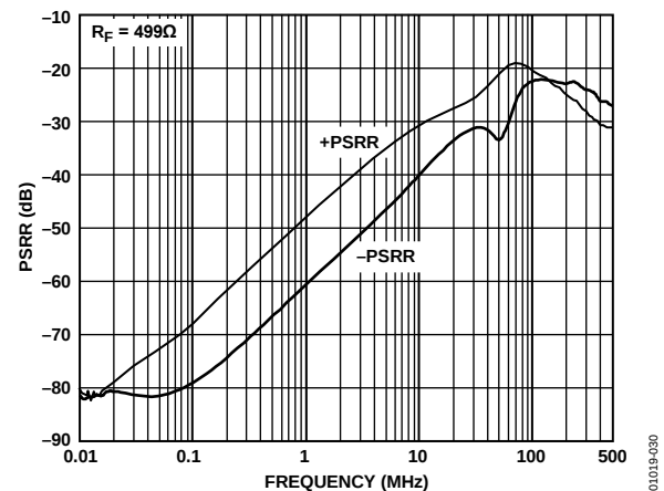
Figure 28. PSRR vs. Frequency; V_S = \pm 12\text{ V}
