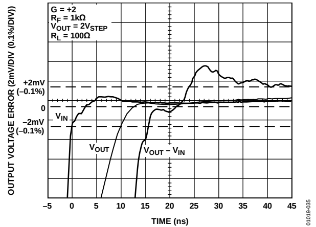
Figure 33. Settling Time 0.1%; V_S = \pm 6\text{ V}
