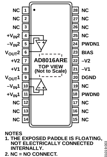
Figure 5. 28-Lead TSSOP_EP (RE-28-1)
