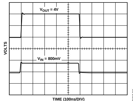
Figure 10. 4 V Step Response; G = +5 , V_S = \pm 12\text{ V} , R_L = 25\ \Omega , Single-Ended
